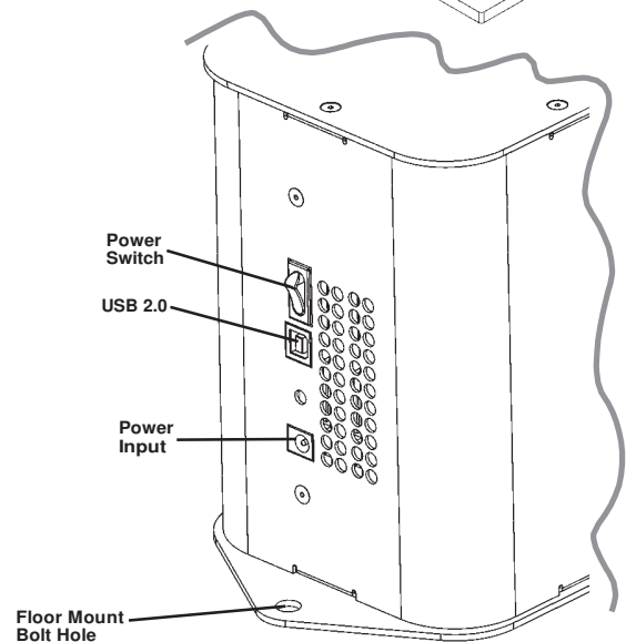
ioSafe Solo Rear Panel
